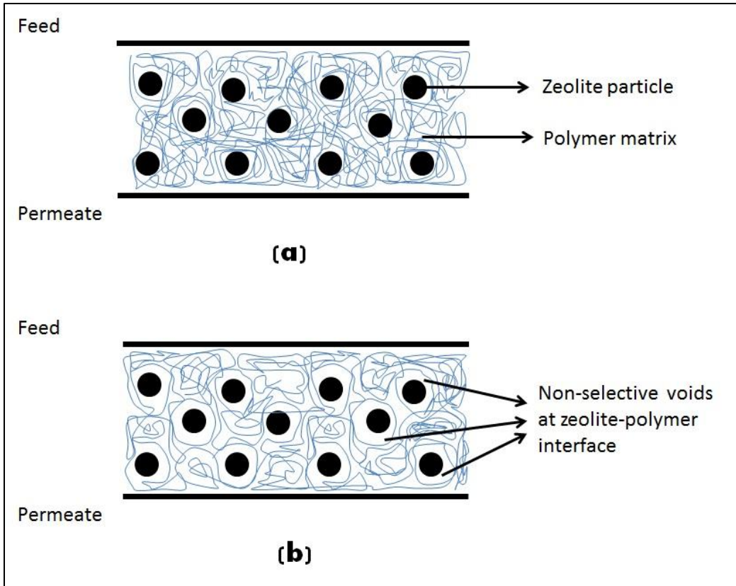
Figure 16 Schematic of (a) densely packed polymer chain matrix at lower temperature (b) increased free volume due to polymer chain mobility and non-selective voids at polymer-zeolite interface occurring at higher temperatures
