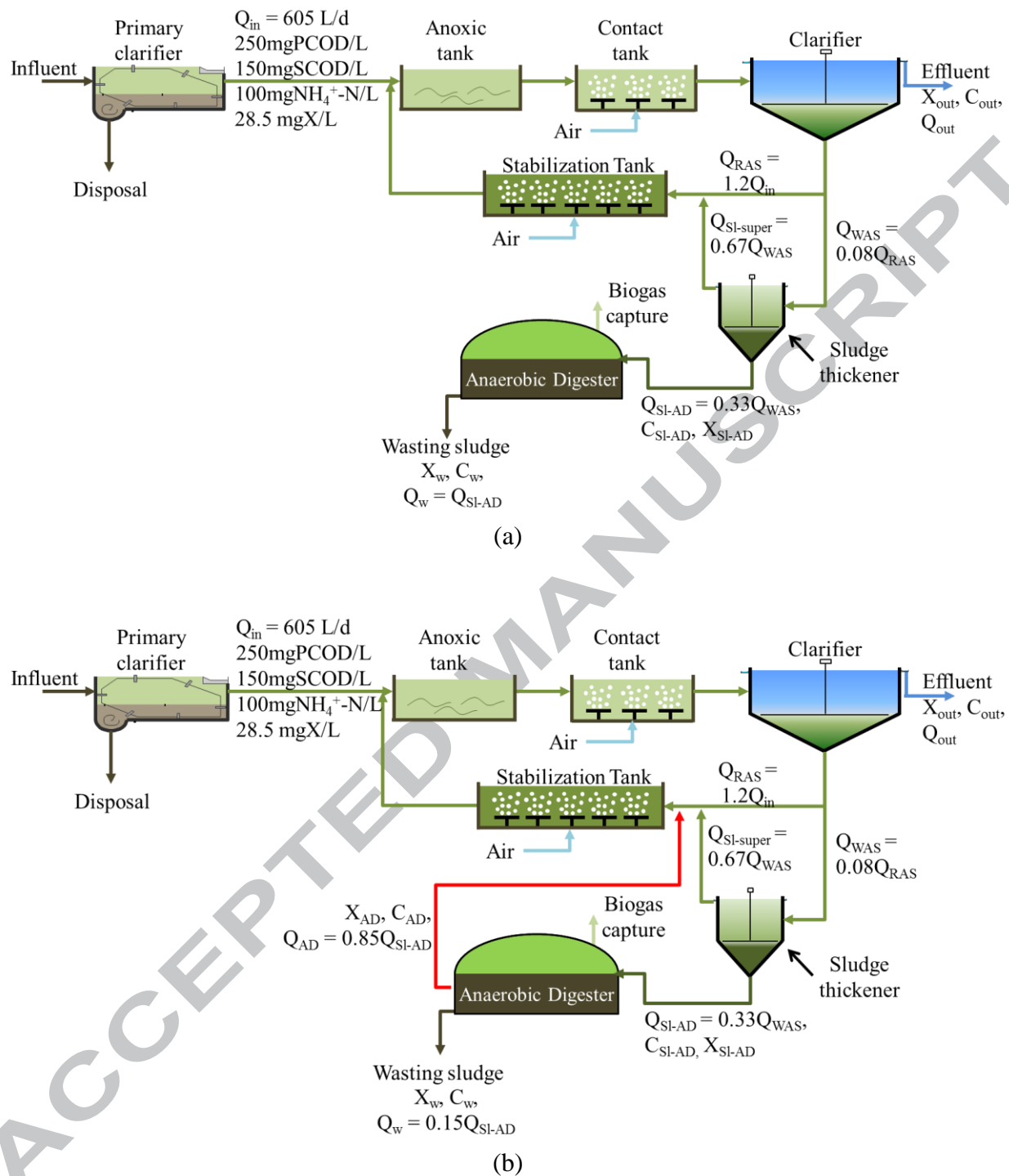
Figure 1. Process configurations modeled: (a) The conventional process. (b) The hybrid process with AD-sludge recycle (heavy red line). Variable labels include Q for volumetric flow rate ( \text{L}^3/\text{t} ), C for concentration ( \text{M/L}^3 ), and X for biomass concentration ( \text{M/L}^3 ). Subscripts represent the influent (in), effluent (out), wasting sludge (w), sludge thickener to AD (SI-AD), and AD (AD). Numerical values indicate input values.
