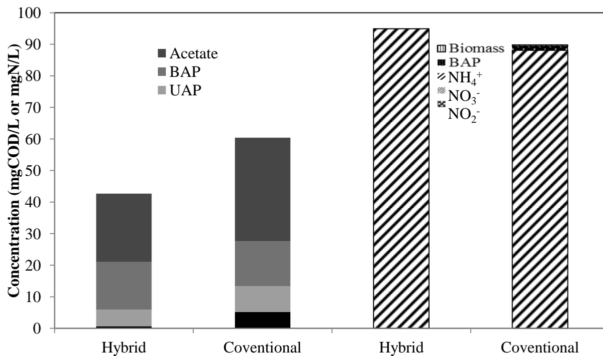
Figure 2. Clarifier-effluent TCOD and TN concentrations in the hybrid and conventional processes. The influent TCOD and TN are 582 mgCOD/L and 116 mgN/L, respectively. The percent TCOD removals are 89.4% for the hybrid system and 88.9% for the conventional system. The percent TN removals are 17% and 26% for the hybrid and conventional systems, respectively.
