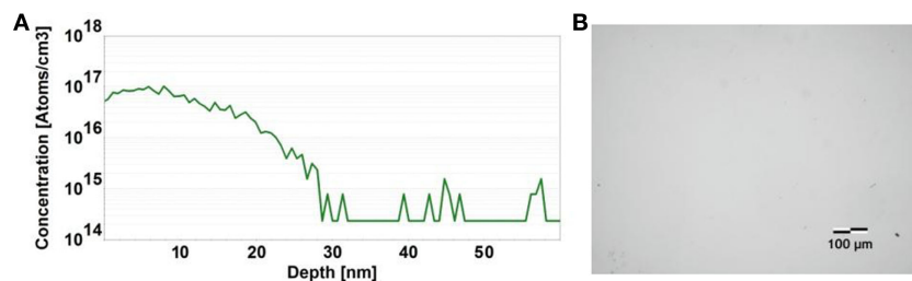
FIGURE 5 | Secondary ion mass spectroscopy profile of a phosphorus-doped diamond film grown on a (100) oriented surface (A) and the corresponding surface morphology acquired via optical microscopy indicating no detectable growth defect formation (B) .
