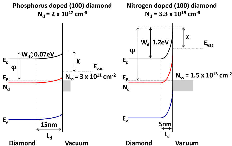
FIGURE 9 | Band bending schematic for single-crystal (100) diamond with different doping concentration of 2 \times 10^{17} \text{ cm}^{-3} for phosphorus-doped diamond and 3.3 \times 10^{19} \text{ cm}^{-3} for nitrogen-doped diamond.
