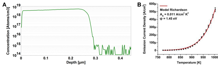
FIGURE 8 | Secondary ion mass spectroscopy profile of a phosphorus-doped diamond film grown on a (111) oriented high-pressure, high temperature type Ib nitrogen-doped diamond surface (A) and the corresponding thermionic electron emission characterization with respect to the Richardson formalism (B) .
