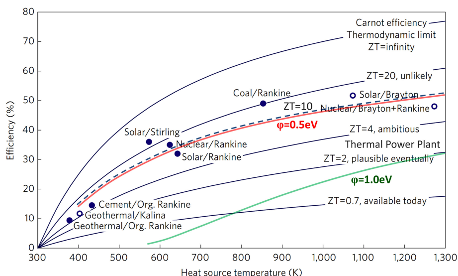
FIGURE 1 | Efficiency for various power generators compared to thermoelectric conversion with figure of merit ZT and thermionic conversion efficiency enabled by low work function collectors (Vining, 2009). With a collector work function of \phi = 1.0 eV efficiencies compare to thermal power plants and for a work function of \phi = 0.5 eV a conversion efficiency of \sim 50\% is possible.
