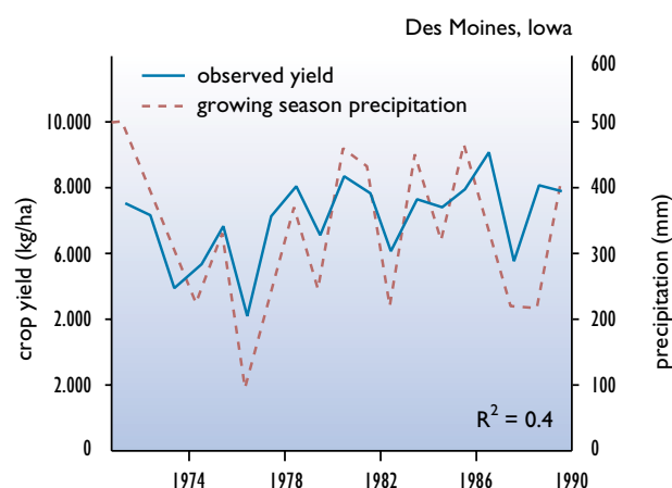
Figure 2 Relationship between corn yield and growing season precipitation in Des Moines, Iowa. (Source: Rosenzweig et al., 2000)
