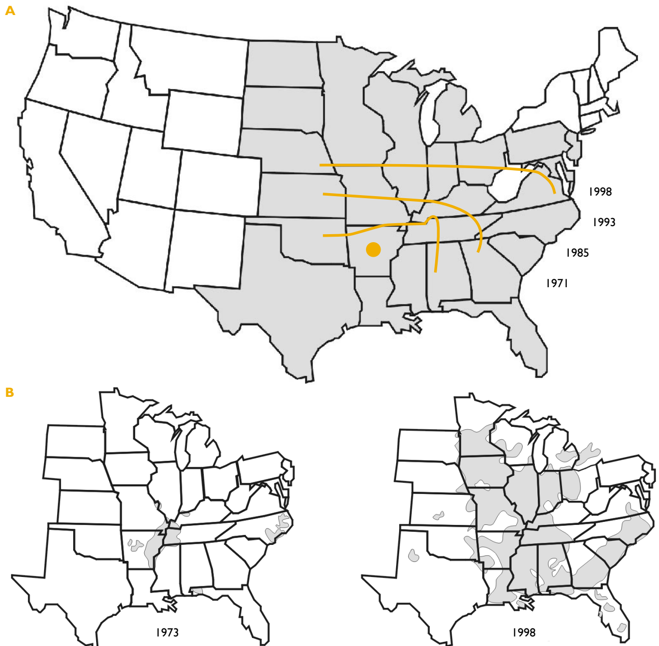
Figure 4 Range expansion of soybean cyst nematode ( Heterodera glycines ) from 1971 to 1998 (A) and soybean sudden death syndrome ( Fusarium solani f. sp. glycines ) from 1973 to 1998 (B) in North America. (Source: Niblack, 1999; X. B. Yang)
