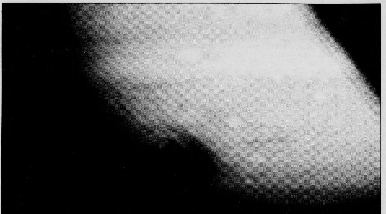
Jupiter shows the scar from the impact of a fragment of the comet Shoemaker/Levy 9. The spot left by the collision is bigger than the planet Earth. Courtesy of NASA
