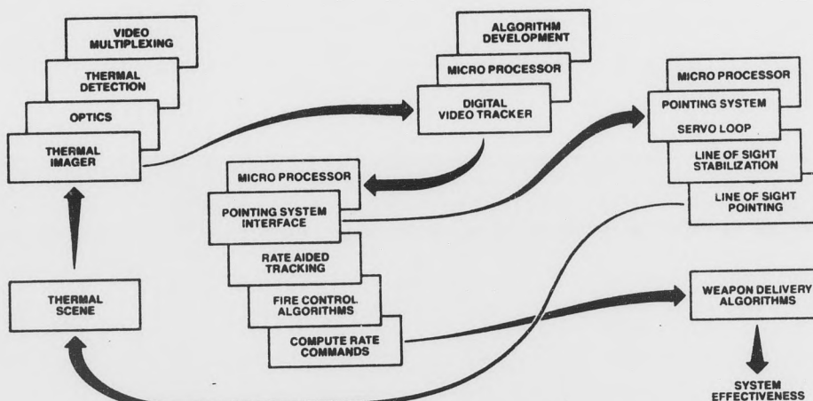
Typical FLIR Fire Control System
