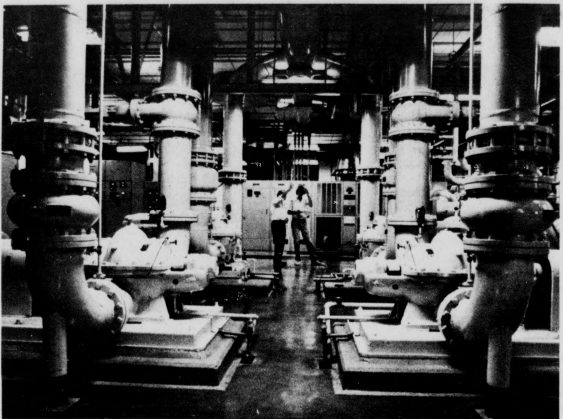
Deep within the Central Plant and surrounded by cooling apparatus, Wilbur German, central plant supervisor, explains the plant operation to a student. The pipes move 3100 gallons-per-minute in order to cool the condensor heads. [State Press staff photo by Sam Jones]
