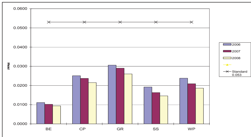
Chart 2 2006-2008 Nitrogen Dioxide Annual Average Readings
