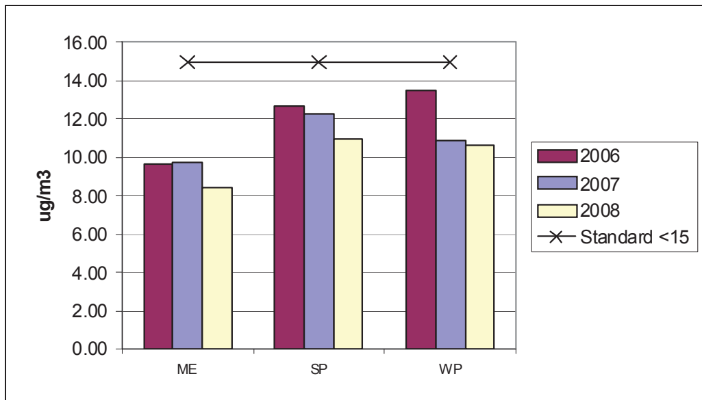
Chart 6 2006-2008 PM 2.5 Annual Average
