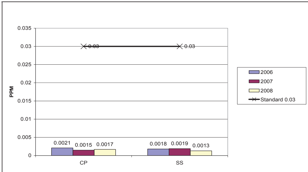
Chart 8 2006-2008 Sulfur Dioxide Annual Average
