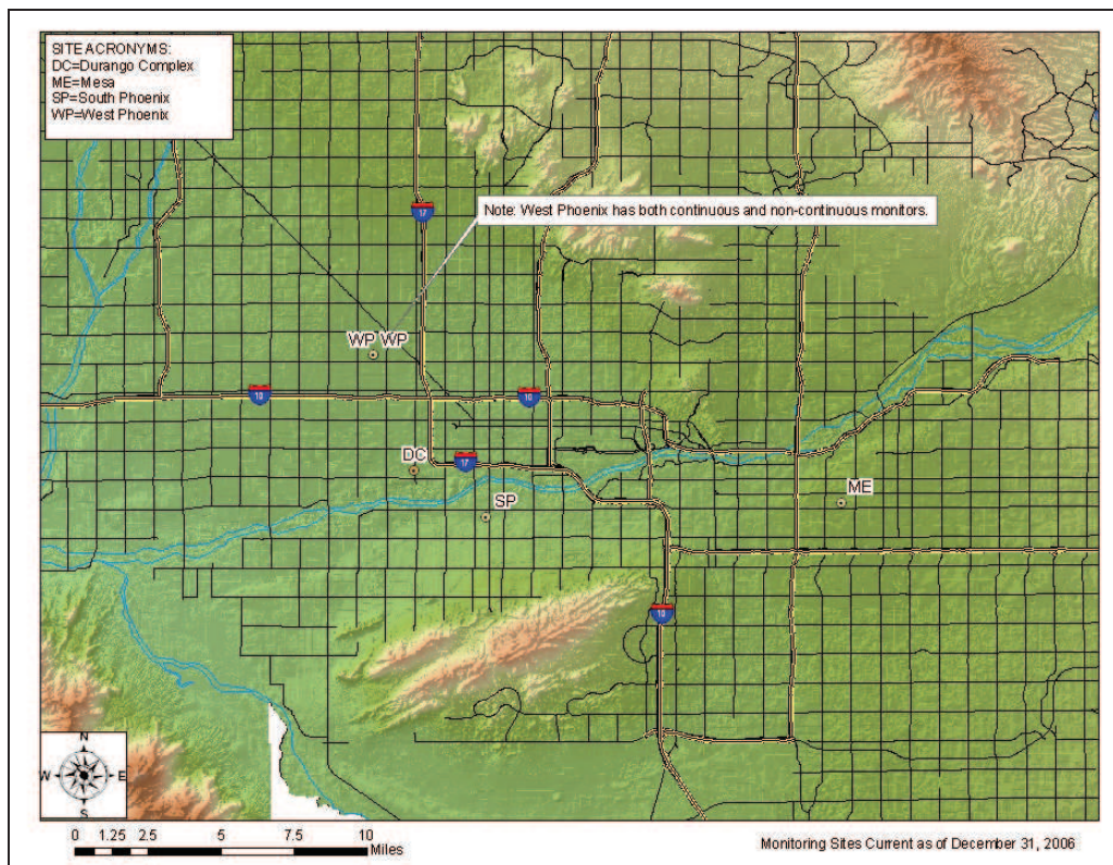
Figure 5 2008 PM_{2.5} Monitoring Sites (continuous and non-continuous)
