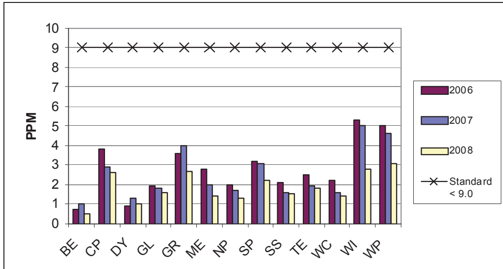
Chart 1 2006-2008 8-hr Avg. Carbon Monoxide Maximum Values
