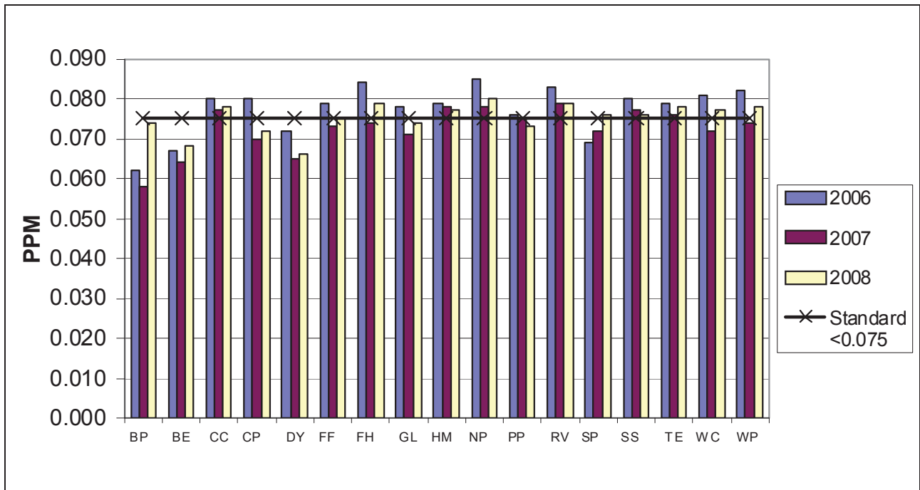
Chart 3 2006-2008 Ozone 4th high 8-hr Average
