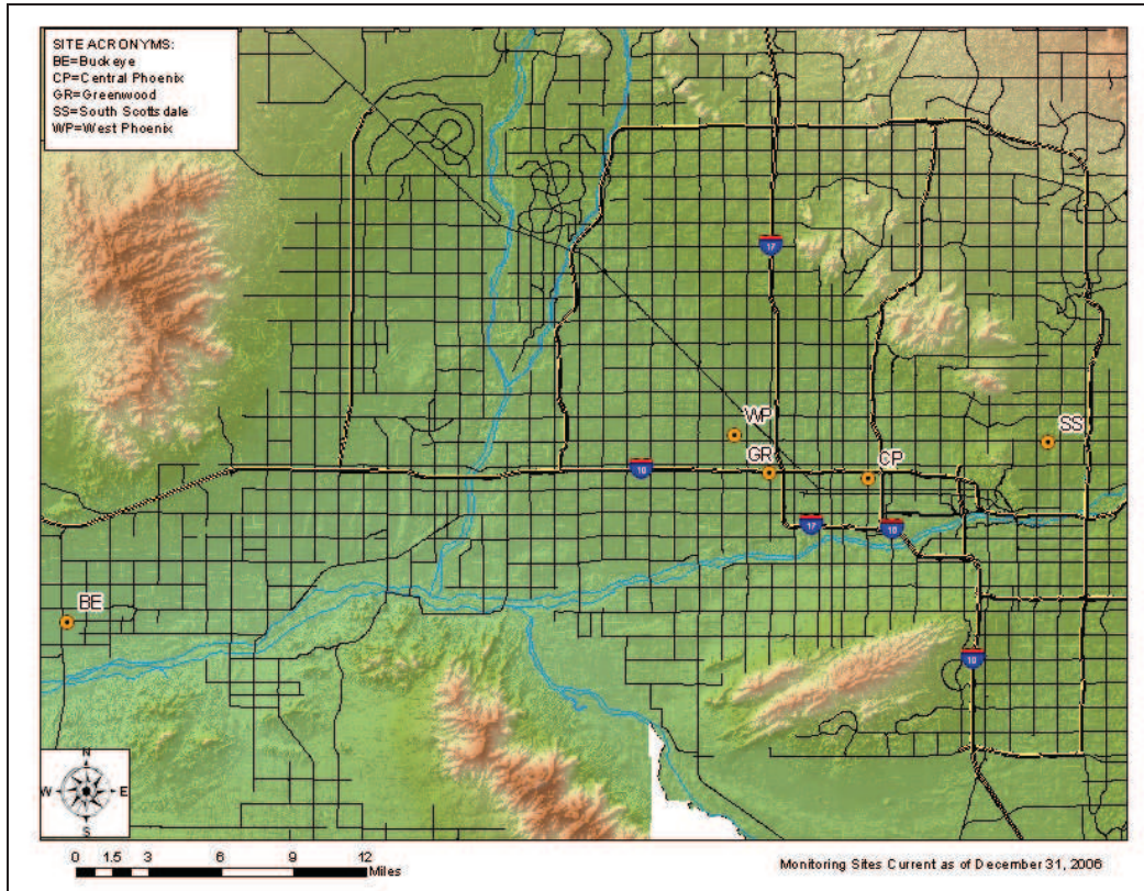
Figure 6 2008 Nitrogen Dioxide Monitoring Sites
