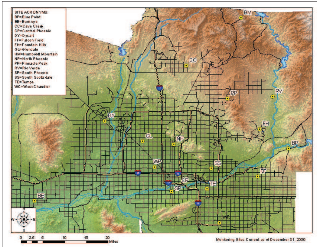
Figure 3 2008 Ozone Monitoring Sites
