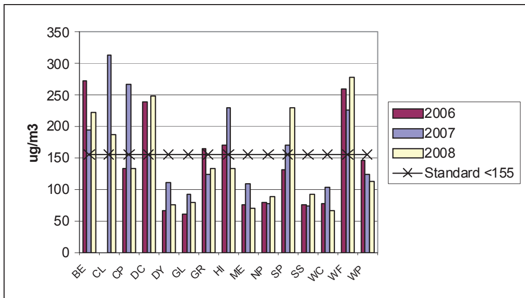
Chart 4 2006-2008 PM 10 24-hr Average Maximum Values
