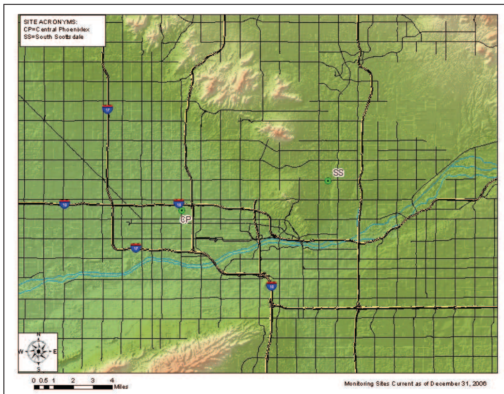
Figure 7 2008 Sulfur Dioxide Monitoring Sites
