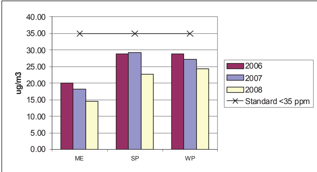
Chart 7 2006-2008 PM 2.5 98 th Percentile
