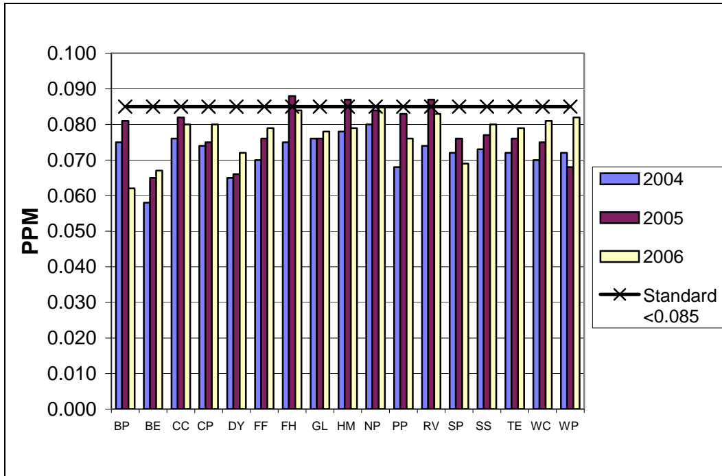
Chart 3 2004-2006 Ozone 4th high 8-hr Average
