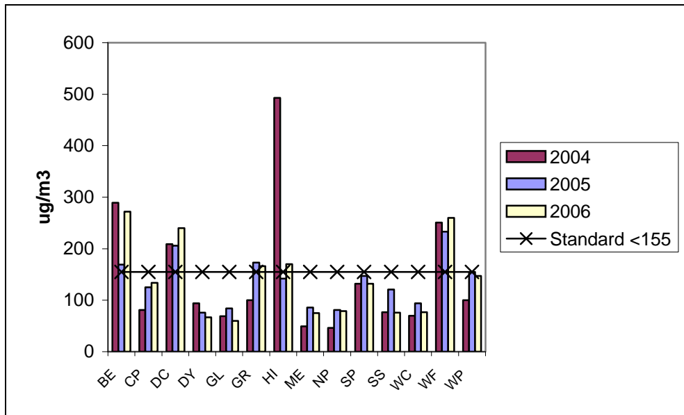
Chart 4 2004-2006 PM-10 24-hr Average Maximum Values
