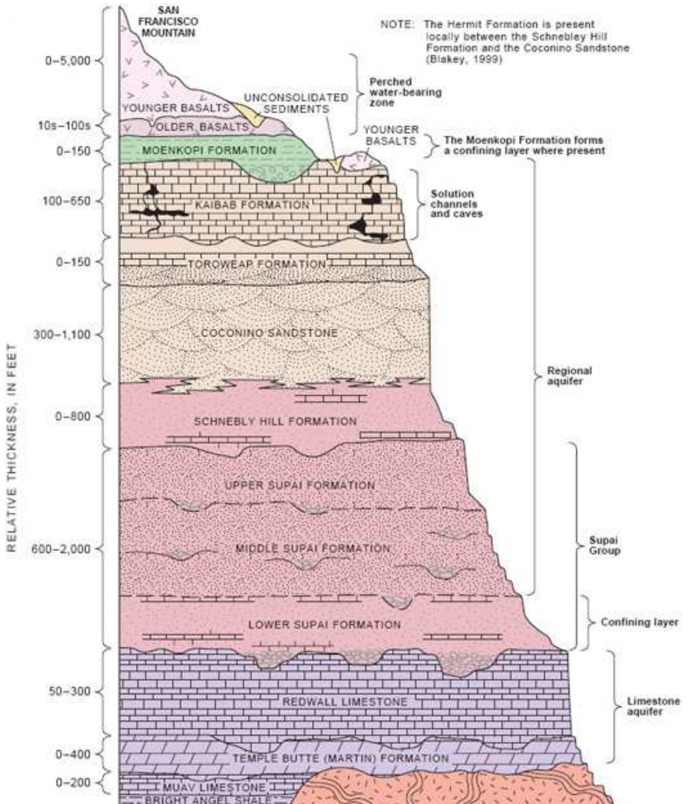
Figure 6.0-5 Generalized stratigraphic section of the Coconino Plateau, Arizona (Bills and Flynn, 2002)
