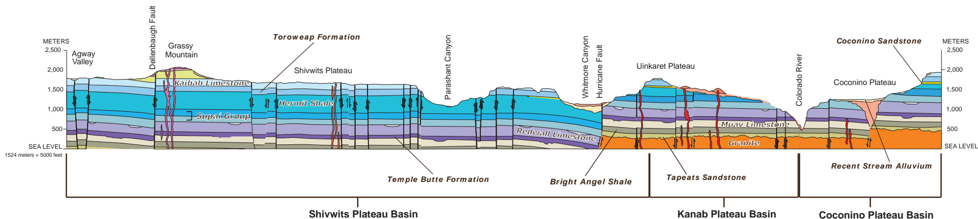
Figure 6.0-6 Geologic cross section of the Shivwits Plateau, Kanab Plateau and Coconino Plateau Basins (modified from Billingsley and Welmeyer, 2003)
