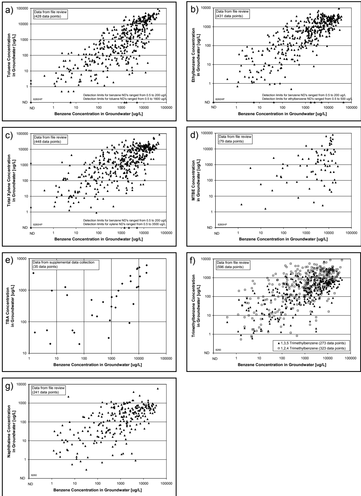
Figure 5.13. Co-occurrence of Chemicals with Benzene in Source Zone Groundwater.
