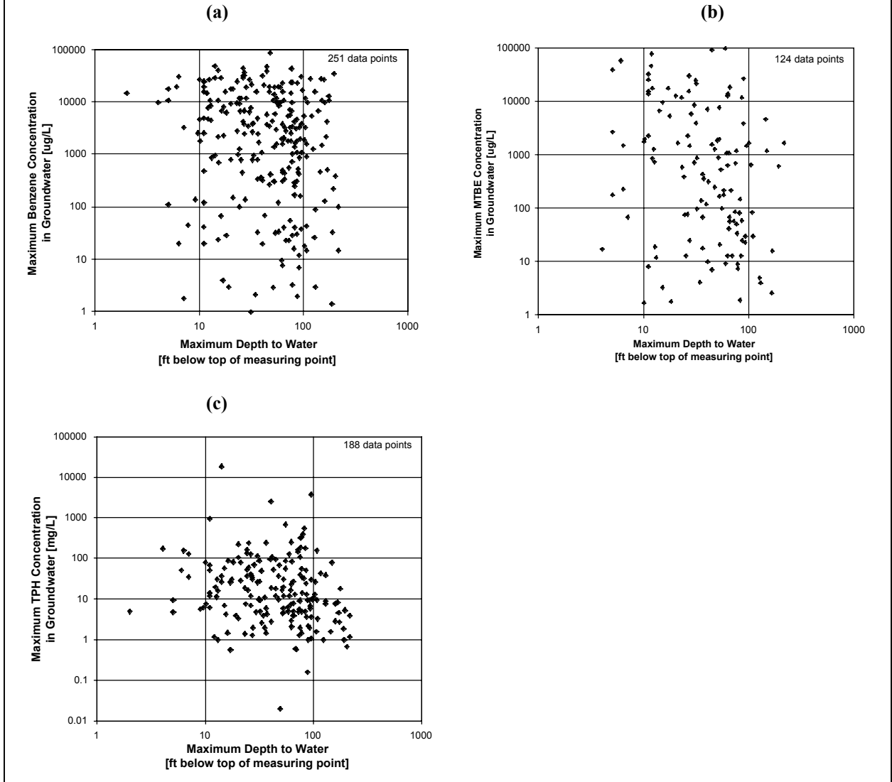
Figure 5.11. Maximum Contaminant Concentration vs. Maximum Depth-to-Water For (a) benzene, (b) MTBE, and (c) TPH.
