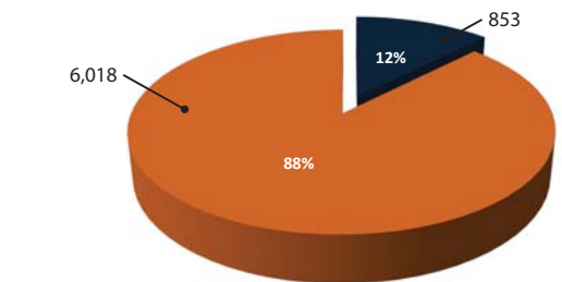
Truck Involved Crashes Compared to Total Crashes in Arizona
