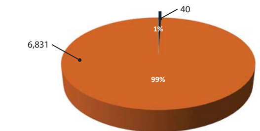
Dust/Wind Related Crashes Compared to Total Crashes in Arizona
