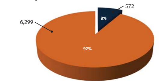
Unhelmeted Motorcyclist Crashes Compared to Total Crashes in Arizona
