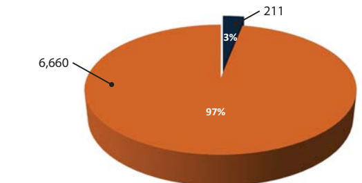
Wet Weather Crashes Compared to Total Crashes in Arizona
