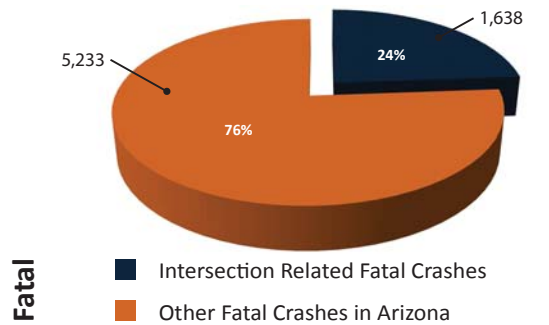
Intersection Related Crashes Compared to Total Crashes in Arizona
