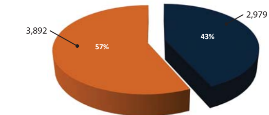
Highway Crashes Compared to Total Crashes in Arizona
