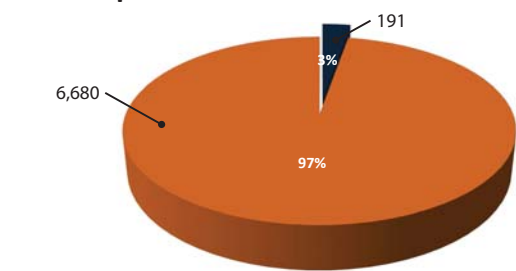
Pedalcyclist Involved Crashes Compared to Total Crashes in Arizona
