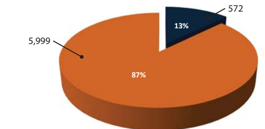
Tribal Land Crashes Compared to Total Crashes in Arizona
