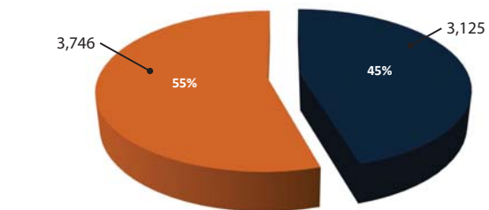
Rural Crashes Compared to Total Crashes in Arizona
