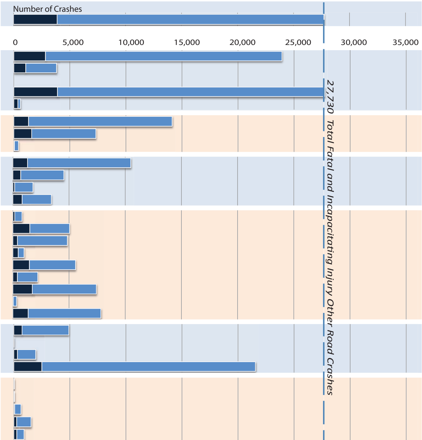
Other Road Fatal and Incapacitating Injury Crash Statistics from 2005-2012
