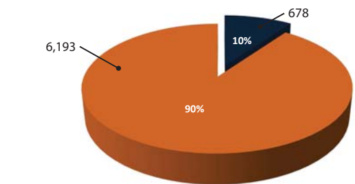
Drug Involved Crashes Compared to Total Crashes in Arizona
