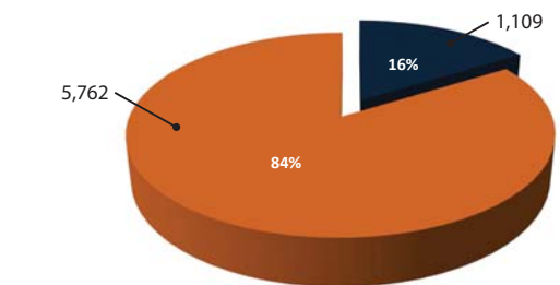
Motorcycle Involved Crashes Compared to Total Crashes in Arizona
