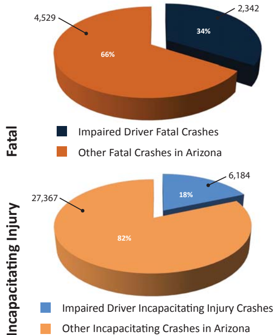
Impaired Driver Crashes Compared to Total Crashes in Arizona
