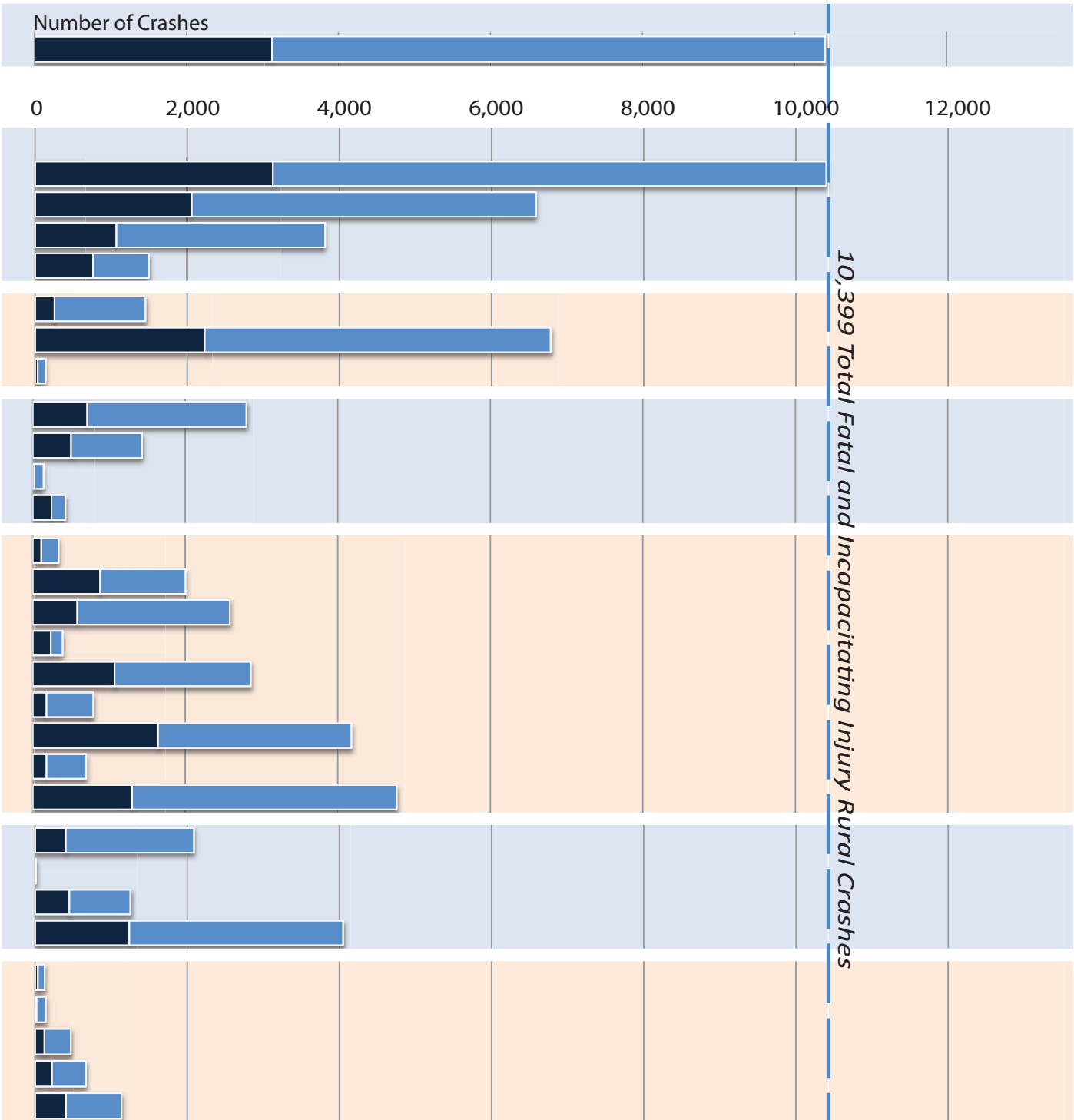
Rural Fatal and Incapacitating Injury Crash Statistics from 2005-2012
