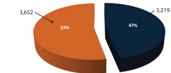
No Restraint Used Crashes Compared to Total Crashes in Arizona
