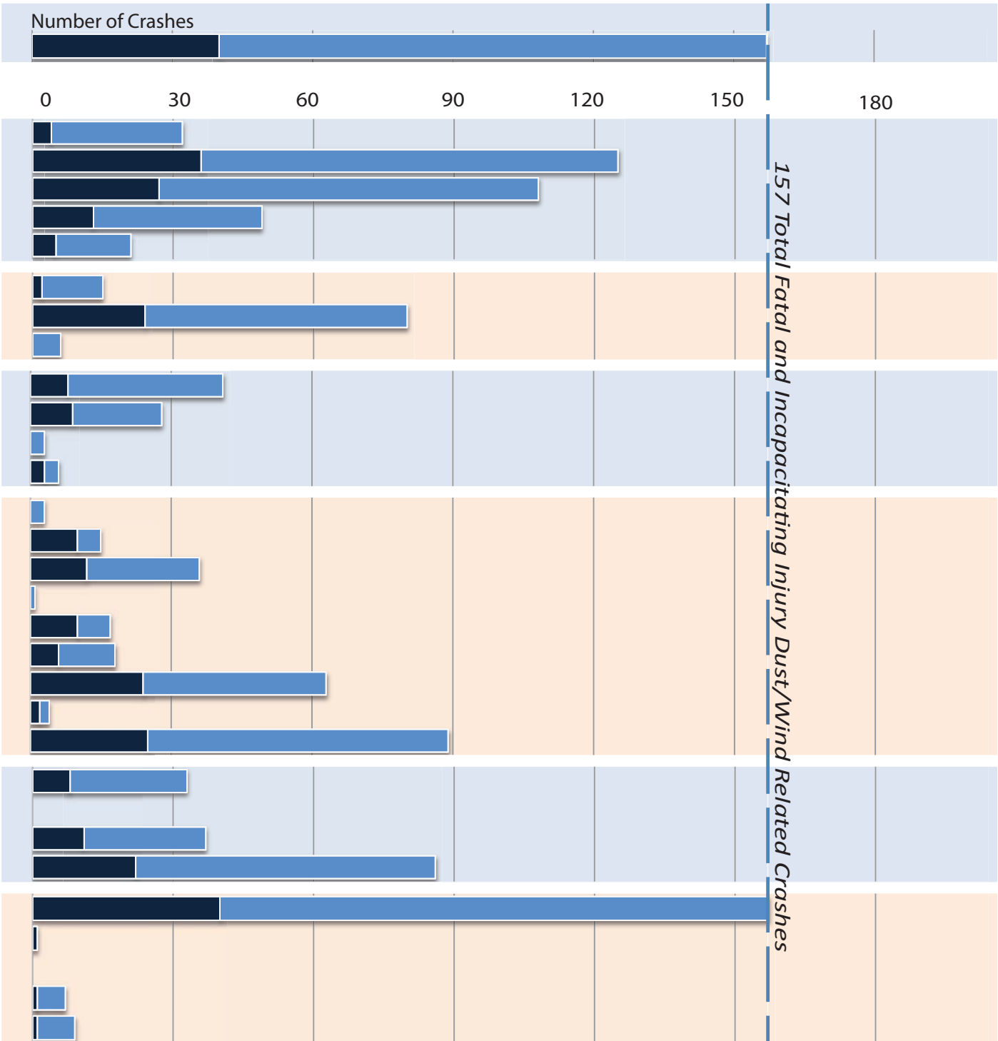
Dust/Wind Related Fatal and Incapacitating Injury Crash Statistics from 2005-2012
