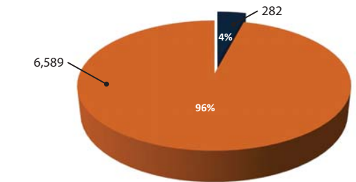
Percent of Aggressive Driver Crashes Compared to Total Crashes in Arizona
