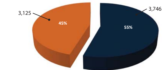
Urban Crashes Compared to Total Crashes in Arizona
