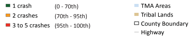
Crash Count per 5-square-mile Area (Distribution Percentile)
