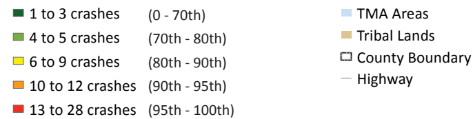
Crash Count per 5-square-mile Area (Distribution Percentile)
