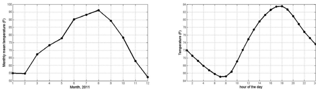
Figure 6.3–1. Monthly averaged temperature (left panel) and annual mean diurnal cycle of temperature (right panel) in 2011.
