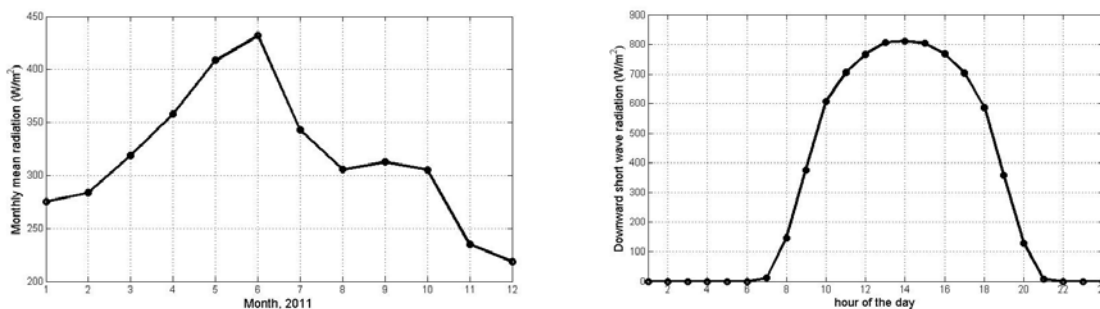
Figure 6.3–2. Monthly averaged radiation (left panel) and annual mean diurnal cycle of radiation (right panel) in 2011.
