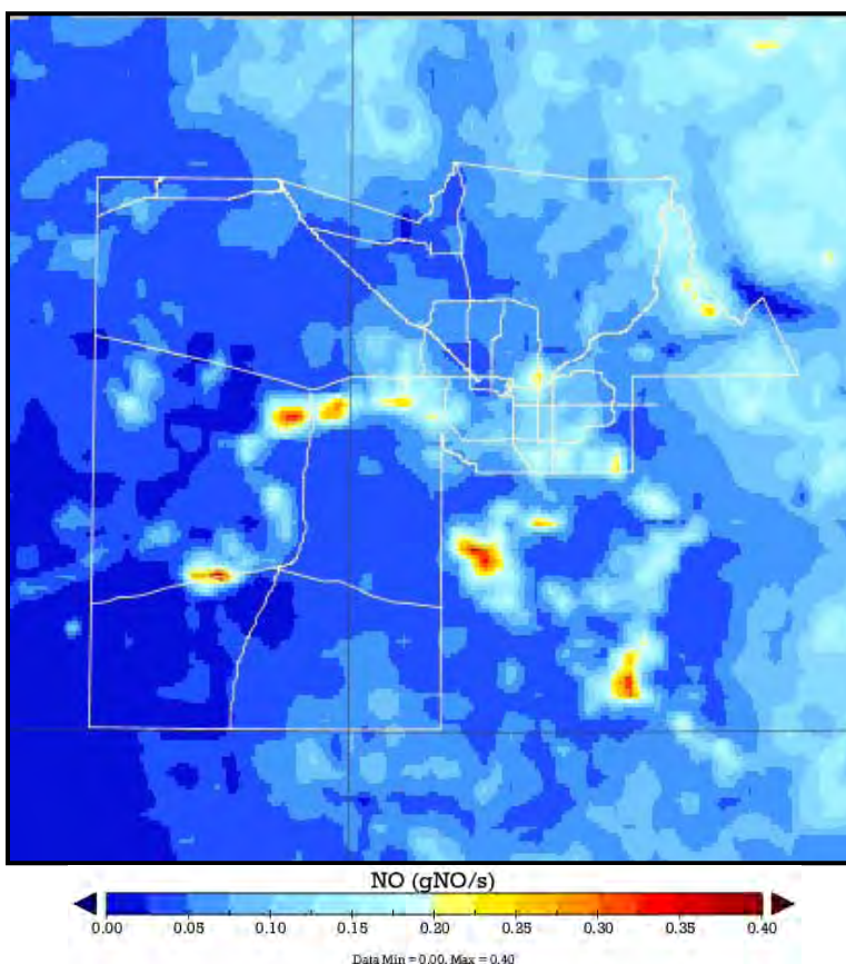
Figure 6.4–1. Estimated emission rates of NO x at 17:00 MST, August 2011 by MEGAN model.
