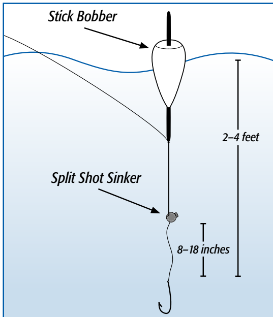
Figure 3: Bobber Setup
