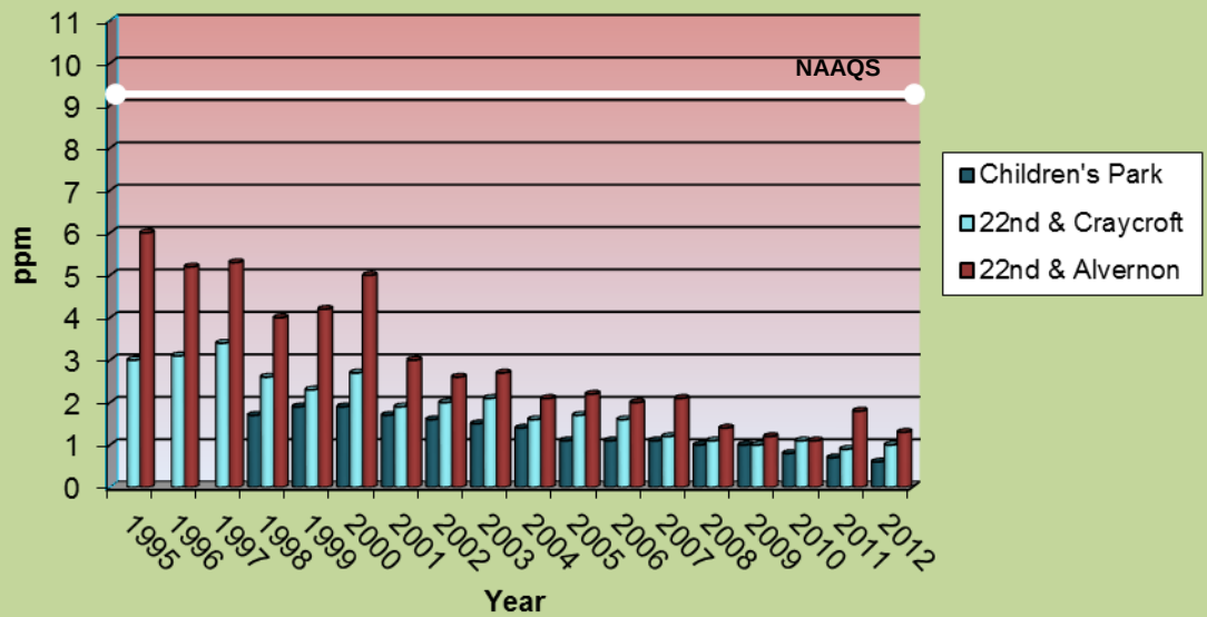
Figure 9 Carbon Monoxide 1995-2012 Highest 8-Hour Average Concentration CO 8-Hour NAAQS = 9 ppm
