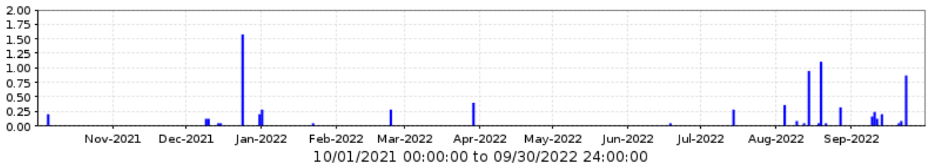
34800 EMF @ Queen Creek Rd. Period Rainfall/1 day
