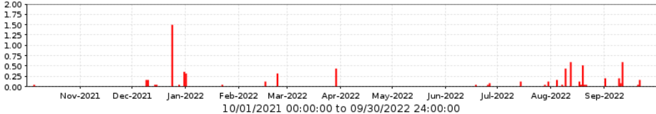
37600 Siphon Draw @ Signal Butte Rd. Period Rainfall/1 day
