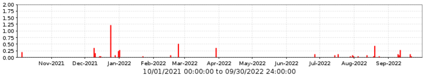
34700 Main St. @ Hawes Rd. Period Rainfall/1 day
