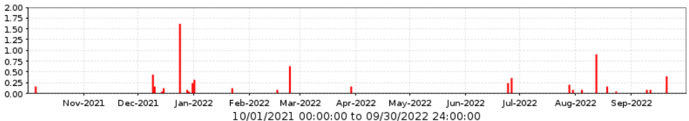
33200 McDowell Rd. @ Hawes Rd. Period Rainfall/1 day
