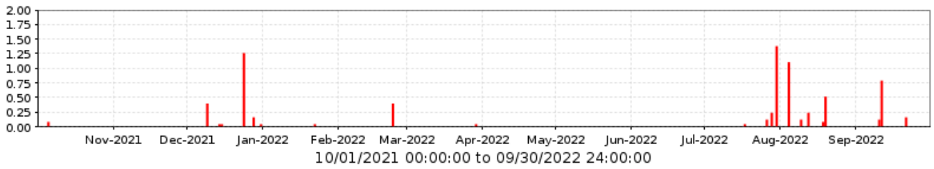
9900 Phoenix Dam 2B Period Rainfall/1 day
