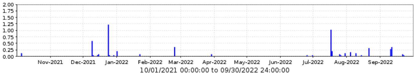
31500 Price Drain @ Loop 202 Period Rainfall/1 day
