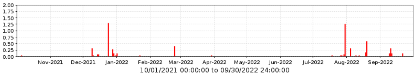
7800 East Fork Cave Cr. Basin #1 Period Rainfall/1 day
