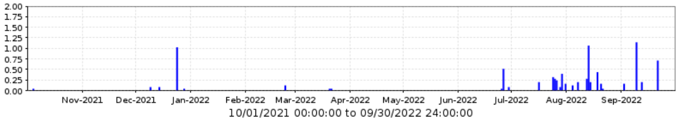
24500 Webb Mountain Period Rainfall/1 day
