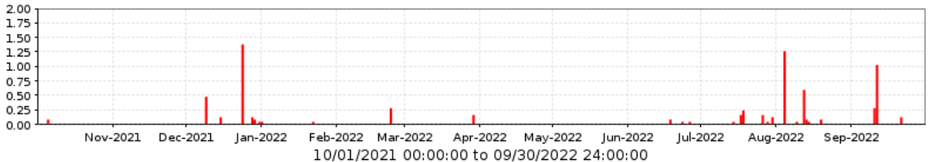
9300 Paradise Valley Country Club Period Rainfall/1 day
