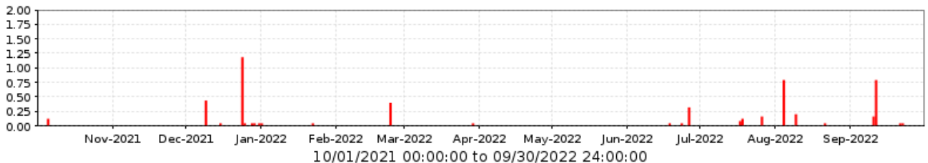
4700 Old Crosscut Canal @ McDowell Rd. Period Rainfall/1 day
