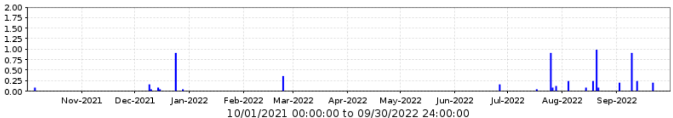
83300 Waterman Wash @ Rainbow Valley Rd. Period Rainfall/1 day
