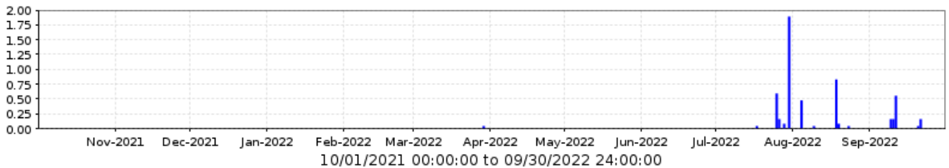
8000 Cave Cr. near Union Hills Dr. Period Rainfall/1 day
