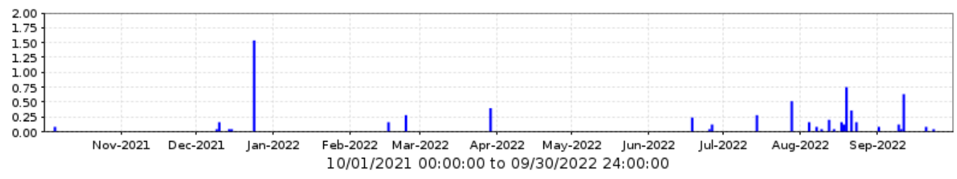
■ 39200 Weekes Wash @ Baseline Rd. Period Rainfall/1 day
