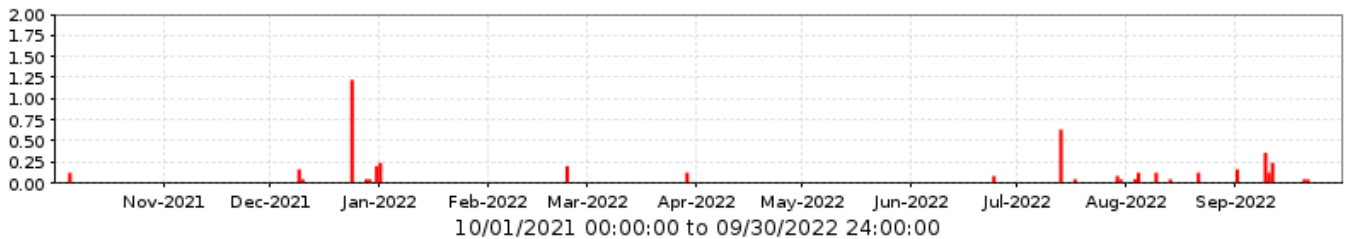
32000 Chandler Blvd. @ Arizona Ave. Period Rainfall/1 day
