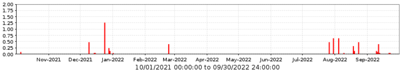
12500 Greenway Rd. @ 32nd Ave. Period Rainfall/1 day
