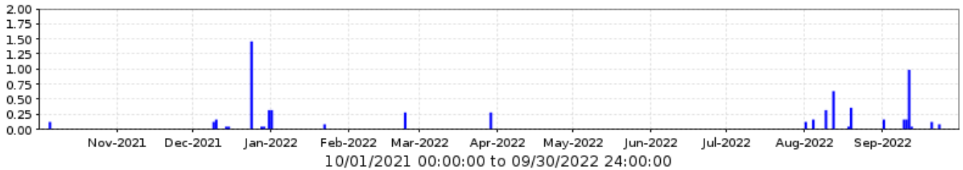
35000 Elliot Rd. @ Loop 202 Period Rainfall/1 day
