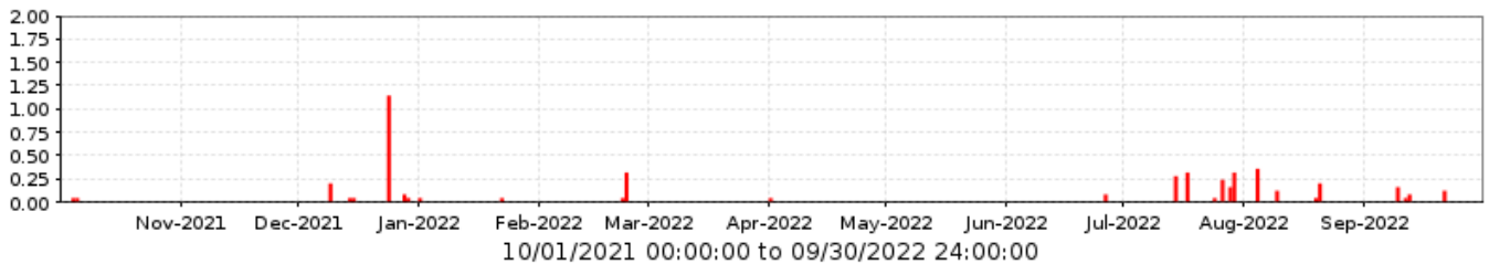
6200 Buckeye Rd. @ 75th Ave. Period Rainfall/1 day
