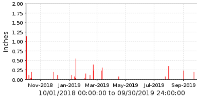
■ 41500 Gila Bend Mountains Period Rainfall/1 day
