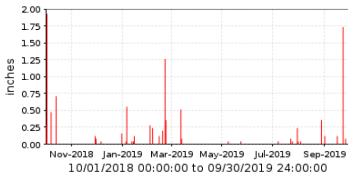
■ 56800 IBW Interceptor Channel Period Rainfall/1 day
