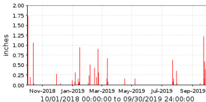
72200 Douglas Ranch Rd. Period Rainfall/1 day
