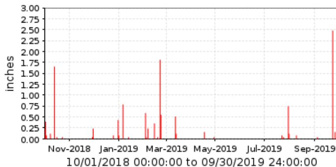
■ 33500 McDowell Rd. @ Meridian Rd. Period Rainfall/1 day
