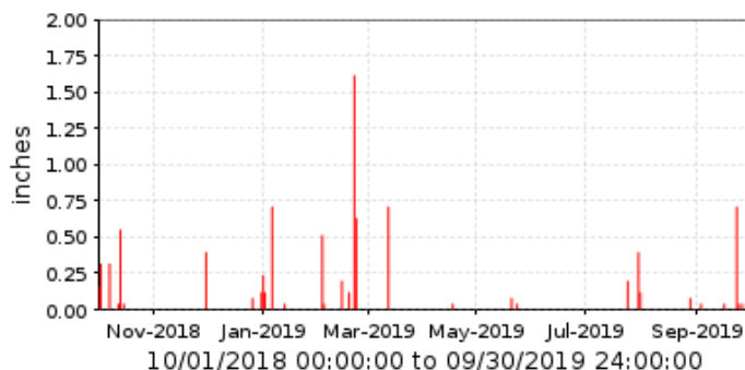
■ 37700 Queen Cr. @ Rittenhouse Rd. Period Rainfall/1 day
