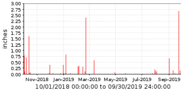
■ 63500 Saguaro Lake Period Rainfall/1 day
