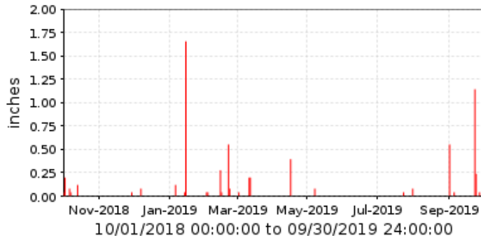
■ 27500 Centennial Wash @ Wenden Period Rainfall/1 day
