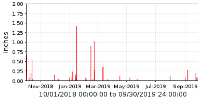
26300 Upper Tiger Wash Period Rainfall/1 day
