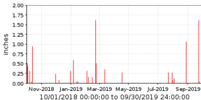
■ 34600 University Dr. @ 62nd St. Basin Period Rainfall/1 day
