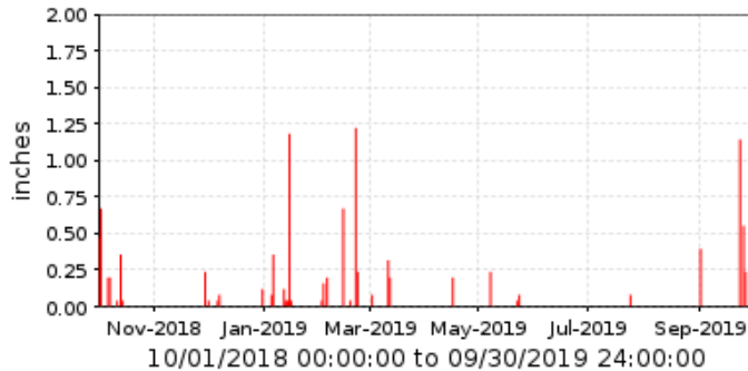
■ 47700 Sols Wash @ SR 71 Period Rainfall/1 day
