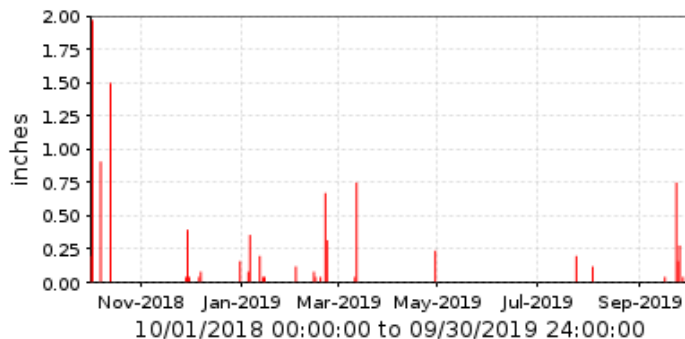
■ 85000 Agua Fria R. @ Buckeye Rd. Period Rainfall/1 day
