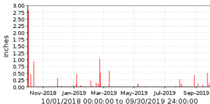
12700 Phoenix Dam #99 Period Rainfall/1 day
