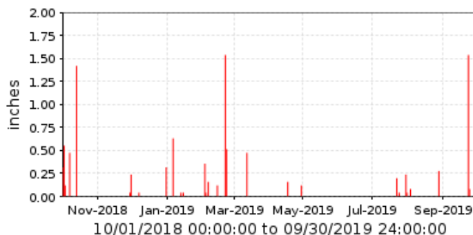
■ 34200 Greenfield Rd. @ Adobe Rd. Period Rainfall/1 day
