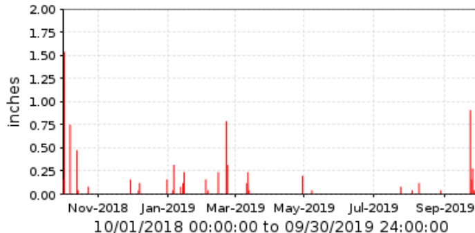
87300 White Tank FRS #3 Period Rainfall/1 day
