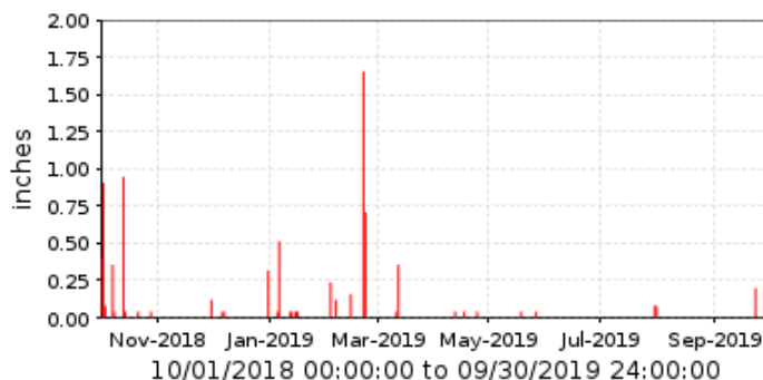
■ 32000 Chandler Blvd. @ Arizona Ave. Period Rainfall/1 day
