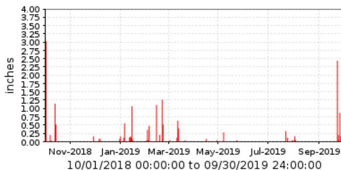
15500 Garfias Mountain Ranch Period Rainfall/1 day
