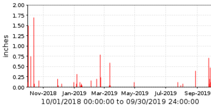
■ 61500 New River @ Glendale Ave. Period Rainfall/1 day
