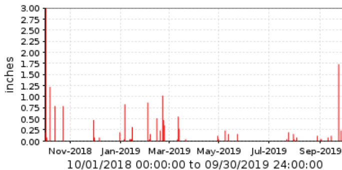
76200 Fraesfield Mountain Period Rainfall/1 day
