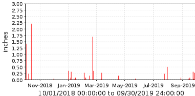
41700 Gila R. @ Maricopa Rd. Period Rainfall/1 day
