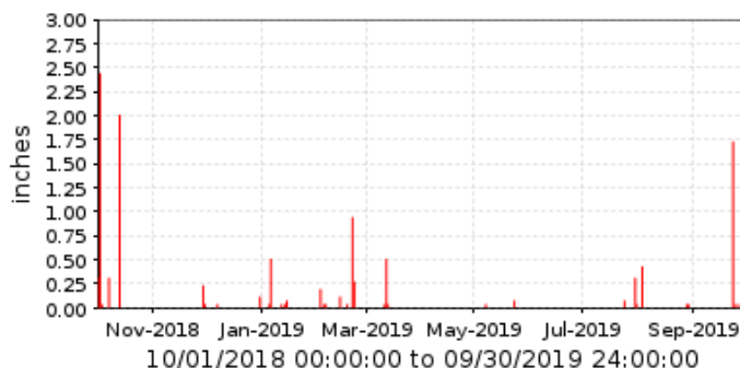
7000 Missouri Ave. @ 16th St. Period Rainfall/1 day
