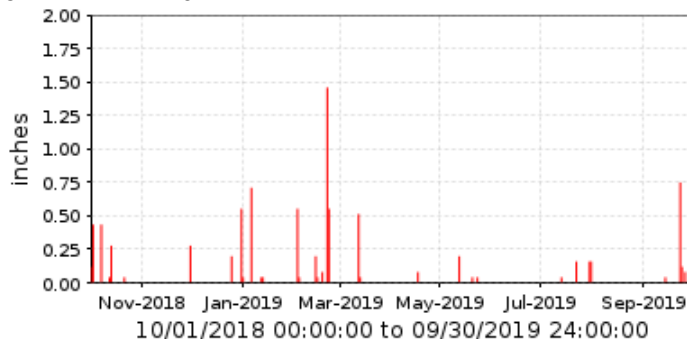
37200 Rittenhouse FRS Period Rainfall/1 day
