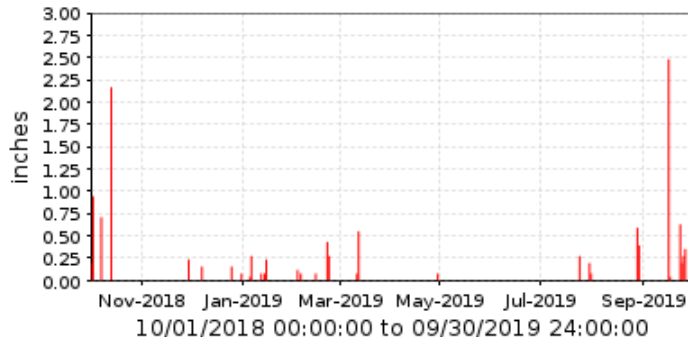
■ 44500 Buckeye FRS #2 Period Rainfall/1 day
