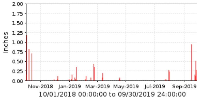
■ 44800 Hassayampa Landfill Period Rainfall/1 day
