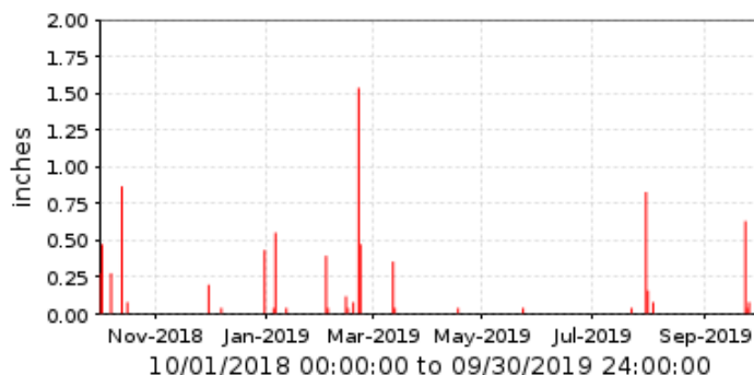
34800 EMF @ Queen Creek Rd. Period Rainfall/1 day
