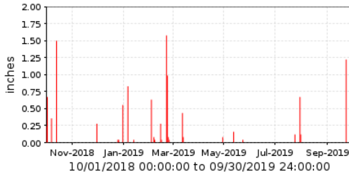
■ 81300 Apache Junction FRS Period Rainfall/1 day
