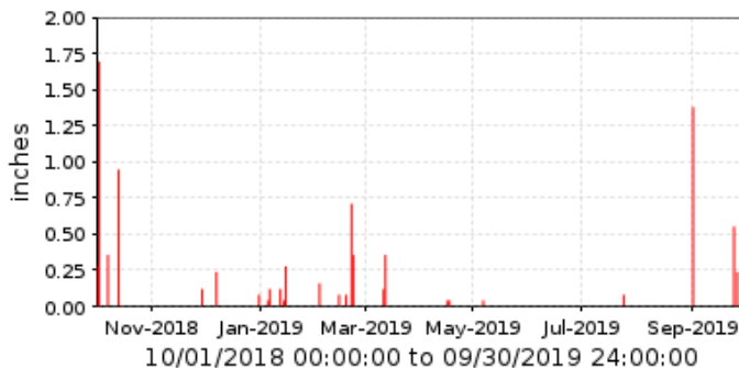
■ 23200 G-F Woolsey Peak Period Rainfall/1 day
