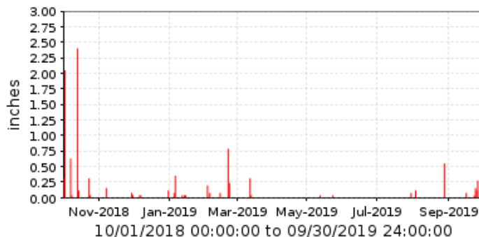
■ 66800 Roeser Rd. @ 23rd Ave. Period Rainfall/1 day
