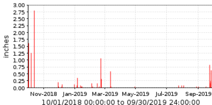
■ 6000 Maryvale Municipal Golf Course Period Rainfall/1 day
