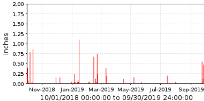
■ 27700 Upper Grass Wash Period Rainfall/1 day
