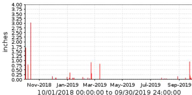
■ 6200 Buckeye Rd. @ 75th Ave. Period Rainfall/1 day
