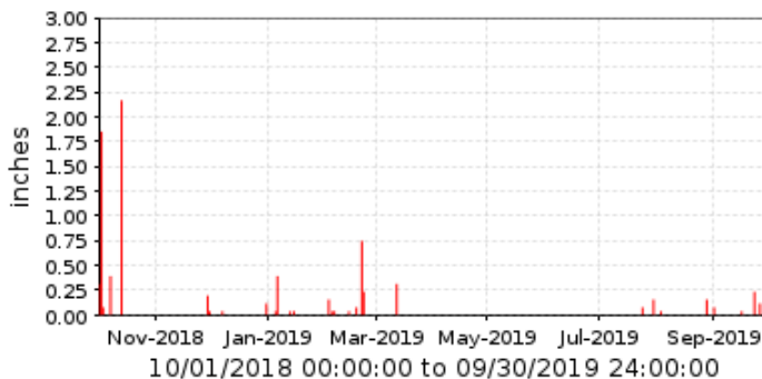
■ 3500 Jackson St. @ 7th Ave. Period Rainfall/1 day
