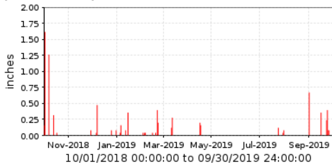
■ 24700 Centennial Railroad Period Rainfall/1 day
