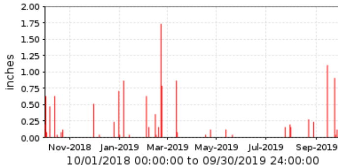
36900 US 60 @ Gold Canyon Period Rainfall/1 day
