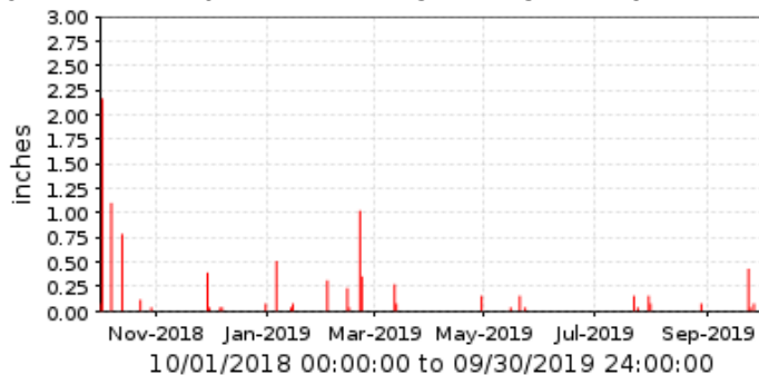
■ 7800 East Fork Cave Cr. Basin #1 Period Rainfall/1 day
