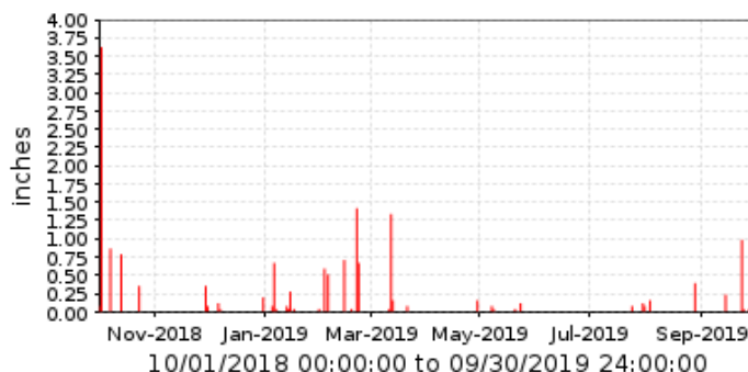
■ 20600 Galloway Wash @ Galloway Rd. Period Rainfall/1 day
