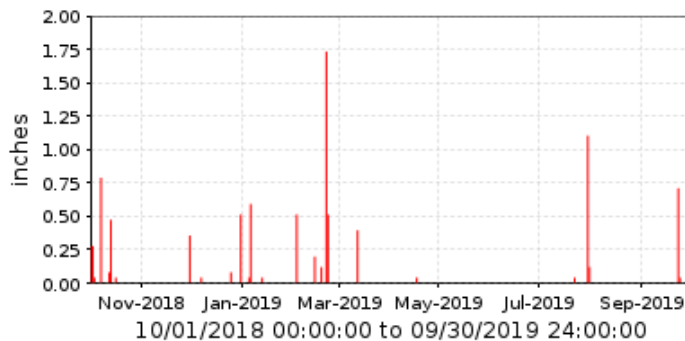
■ 36300 Sonoqui Wash near Hawes Rd. Period Rainfall/1 day
