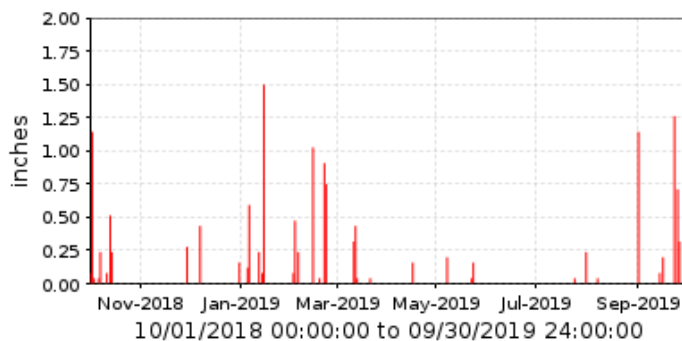
■ 55500 Upper Martinez Cr. Period Rainfall/1 day
