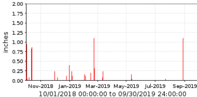
64200 Tat Momolikot Dam Period Rainfall/1 day
