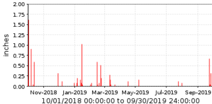
45000 Jackrabbit Wash Period Rainfall/1 day
