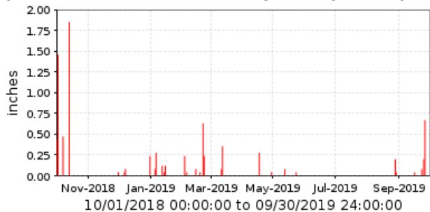
■ 84200 Estrella Fan Period Rainfall/1 day
