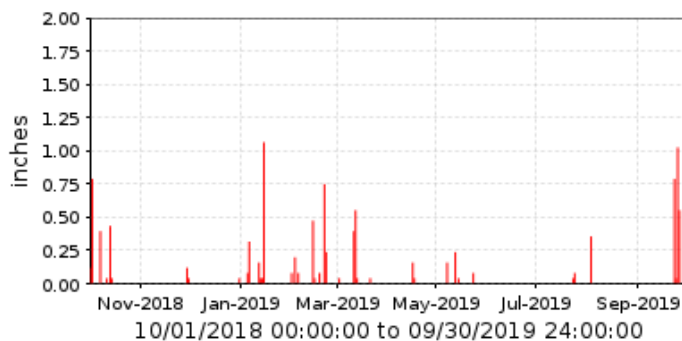
■ 52800 Wickenburg Airport Period Rainfall/1 day
