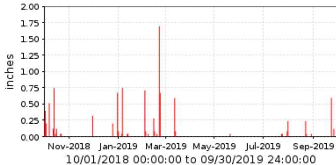
■ 38500 Florence Junction Period Rainfall/1 day
