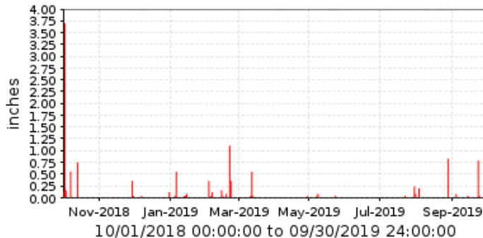
■ 59500 IBW @ Shea Blvd. Period Rainfall/1 day
