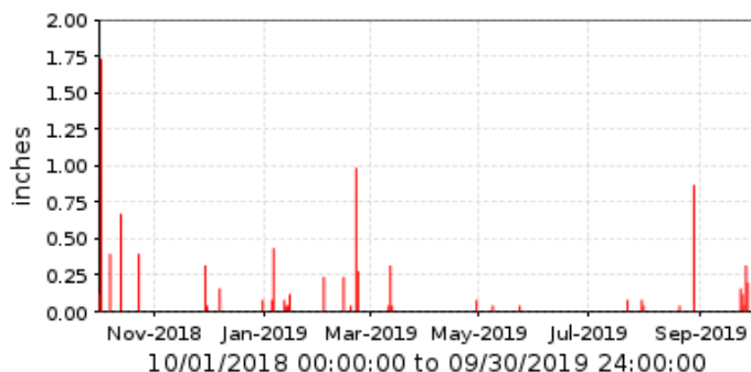
■ 13700 Paradise Lane @ 47th Ave. Period Rainfall/1 day
