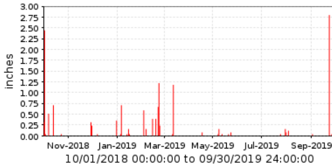
77800 Cloudburst Wash Period Rainfall/1 day
