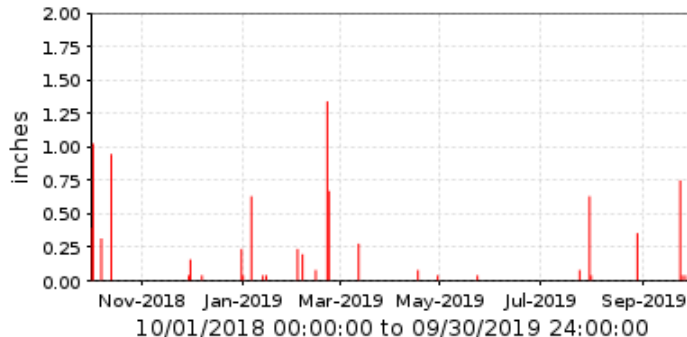
30900 Horne Rd. @ 8th Ave. Period Rainfall/1 day
