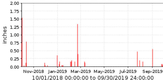
40300 Sand Tank Wash Period Rainfall/1 day
