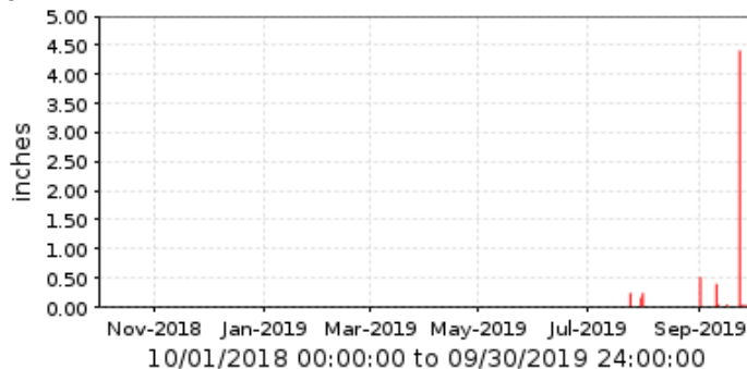
■ 63700 Reavis Trailhead Period Rainfall/1 day
