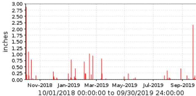
77100 Camp Cr. @ Bartlett Lake Rd. Period Rainfall/1 day
