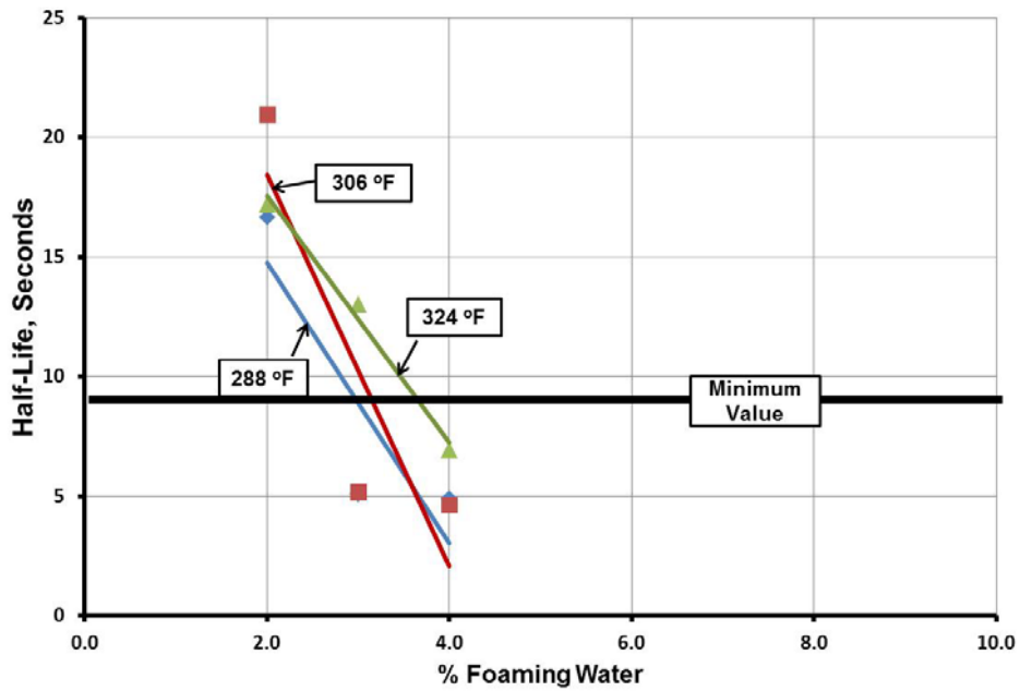
Figure C - 2. PG 64-22 Half-Life
